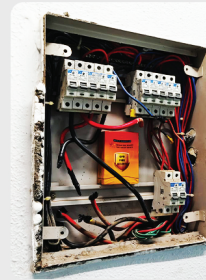
GFO EB(Electric Board) Device
